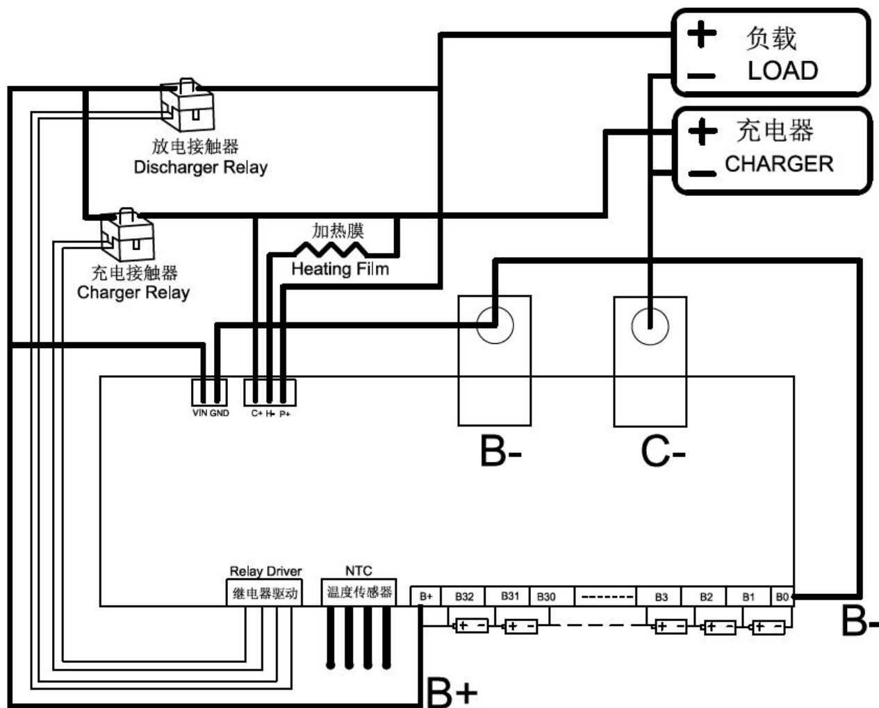
JK-B2A32S-RP-32S接线图 JK-B2A32S-RP-32S wiring diagram
