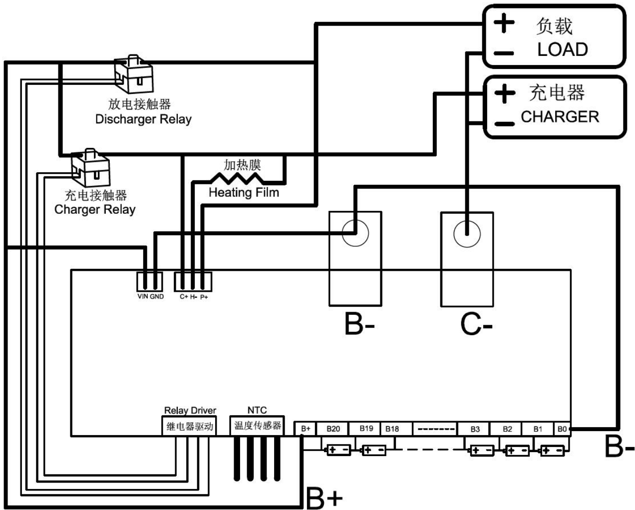
JK-B2A32S-RP-20S接线图 JK-B2A32S-RP-20S wiring diagram
