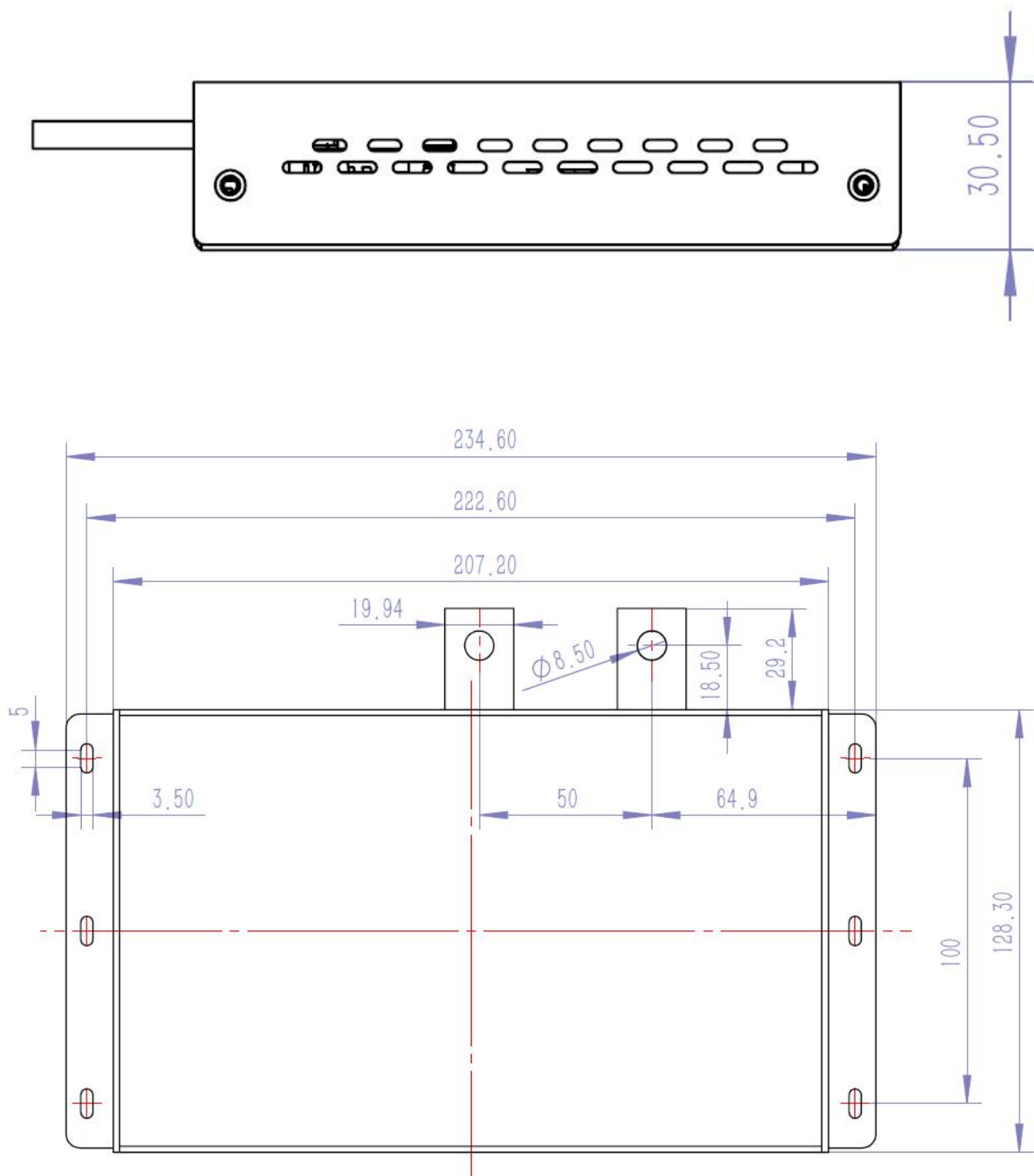
JK-B2A32S-RP 外形尺寸 Dimensions of JK-B2A32S-RP
