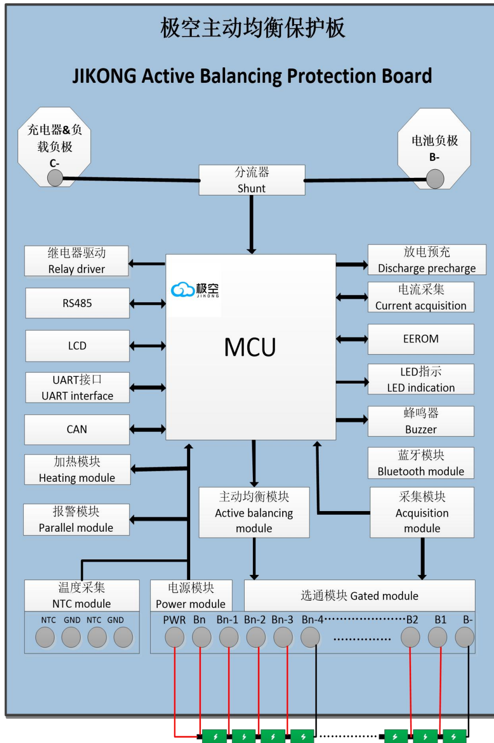
JK-B2A32S-RP 结构框图 JK-B2A32S-RP structure block diagram
