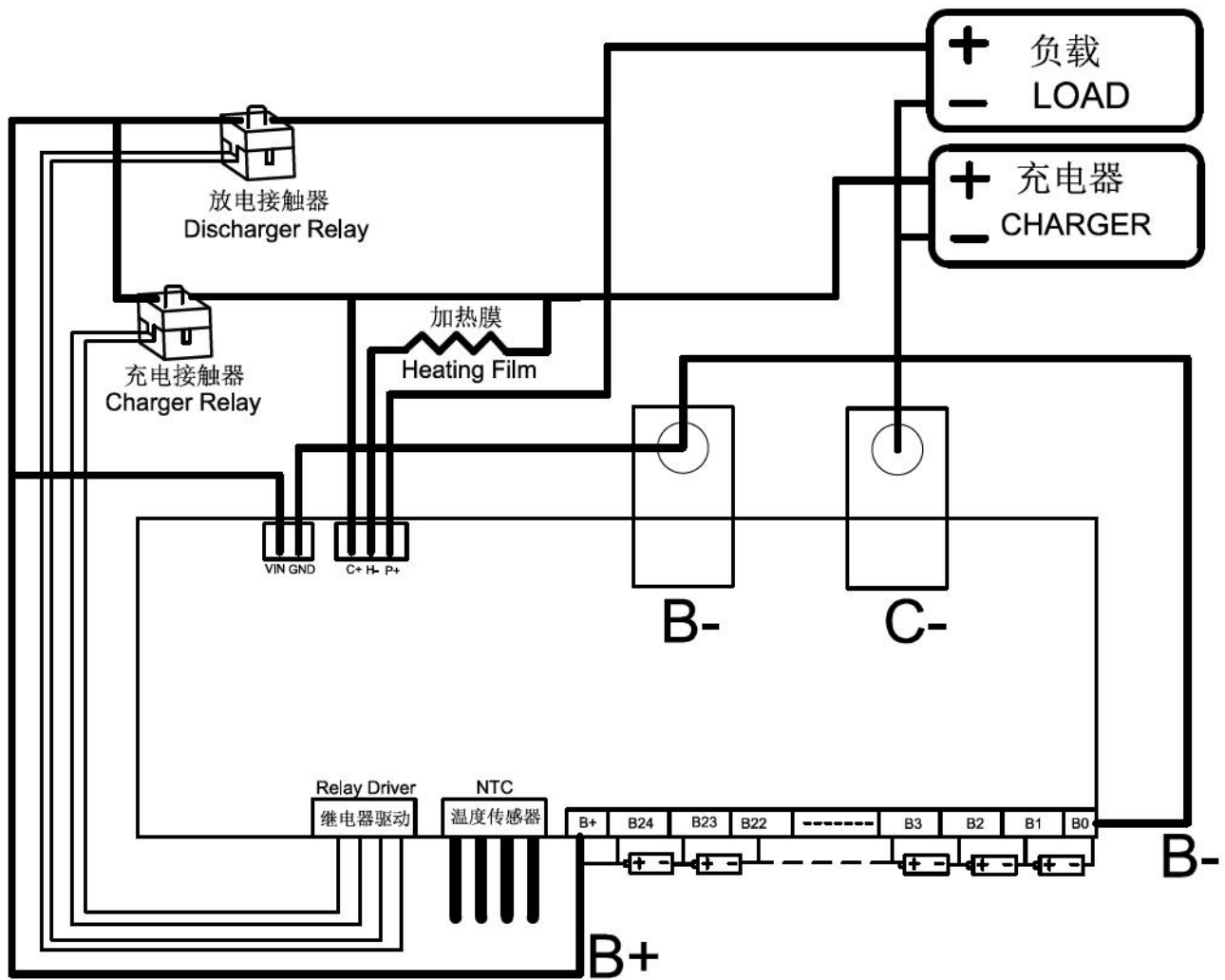
JK-B2A32S-RP-24S接线图 JK-B2A32S-RP-24S wiring diagram
